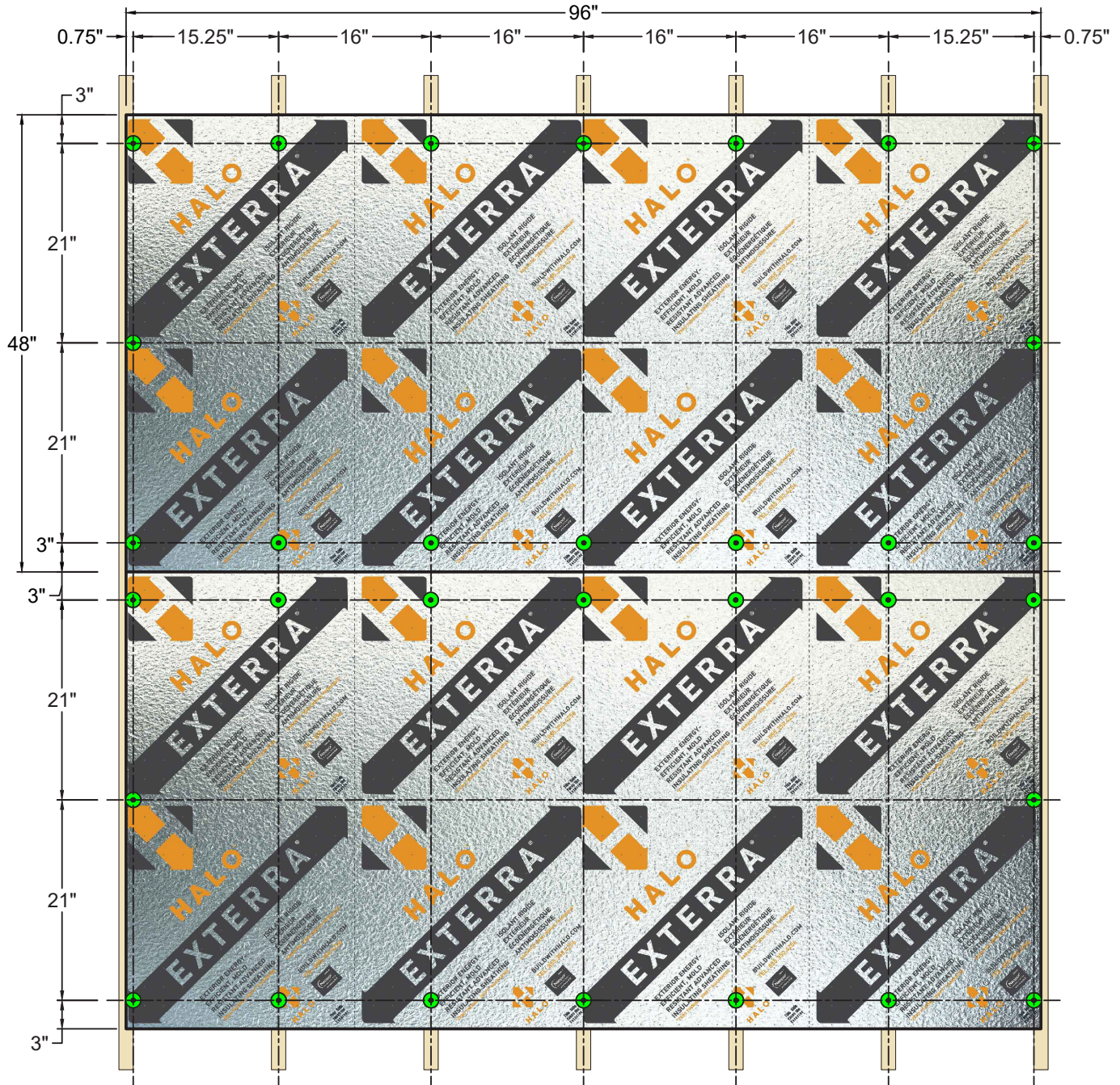
Nailing pattern - Horizontal placement against 16" wood stud spacing (4'x8' Exterra boards shown). Printed guidelines on Exterra boards can be used to locate studs.
