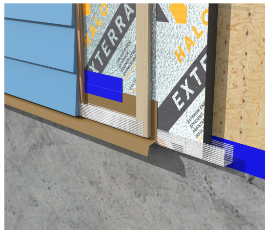
Foundation transition detail without trim board
