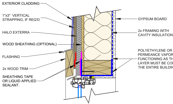
HALO HEADER DETAIL EXAMPLE
