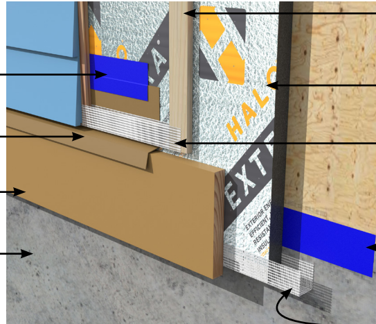
Foundation transition detail with trim board
