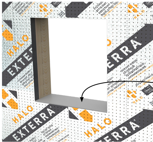
Install back dam and sloped sill.
