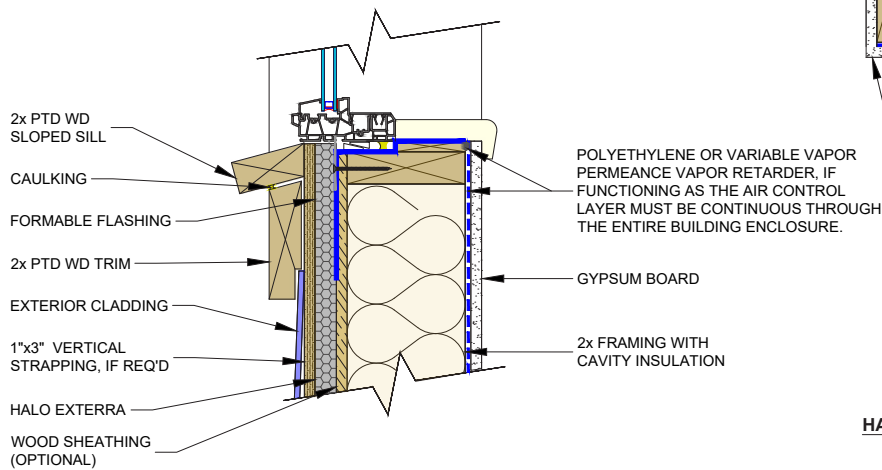
HALO SILL DETAIL EXAMPLE
