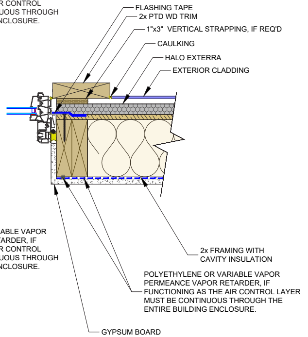
HALO JAMB DETAIL EXAMPLE
